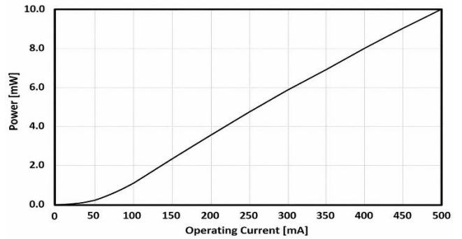
FIG. 2: BTF PACKAGE OUTPUT POWER VS CURRENT
