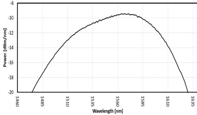
FIG. 1: BTF PACKAGE SPECTRUM
