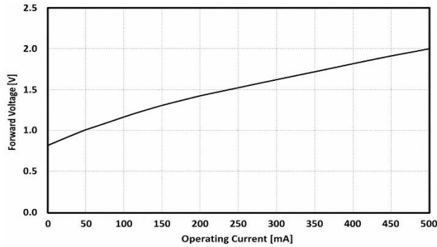
FIG. 3: BTF PACKAGE FORWARD VOLTAGE VS CURRENT
