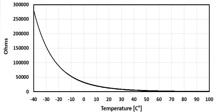
FIG. 4: THERMISTOR R_{THTEC} RESISTANCE VS TEMP.
